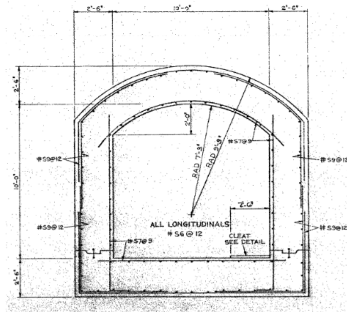
Section view of the tunnel
