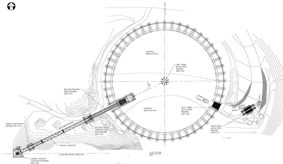
Site layout of alumina silos & reclaiming system for alumina silo 775-4
