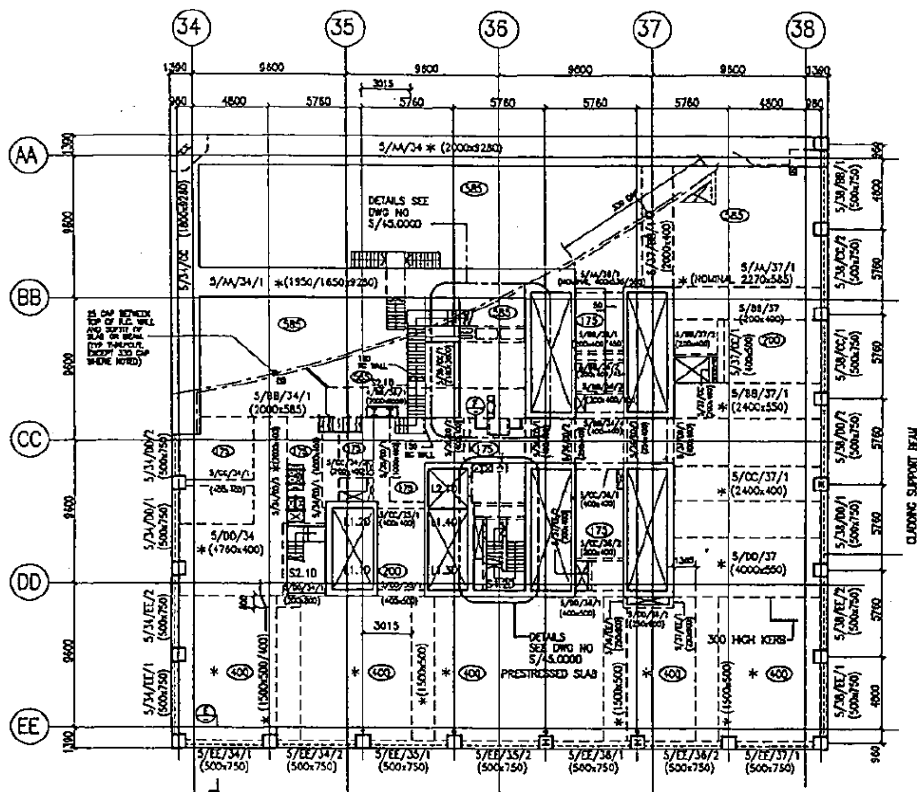
Layout of the transfer floor
